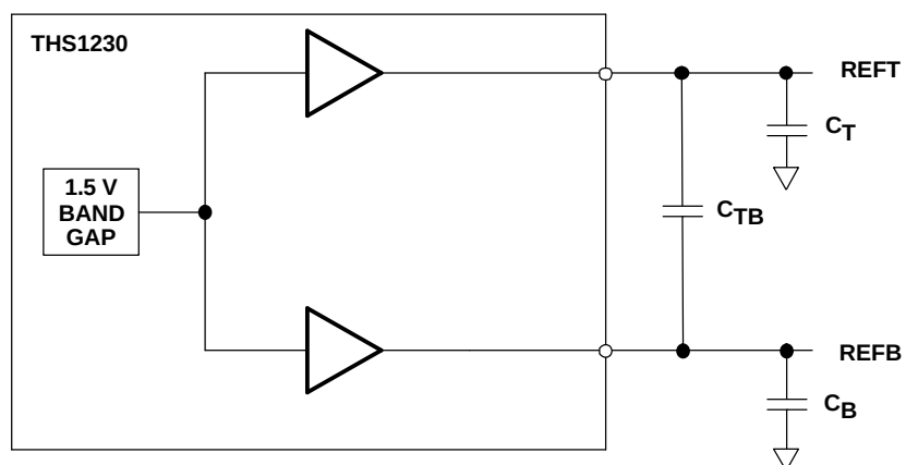
Figure 1. Reference Generation
